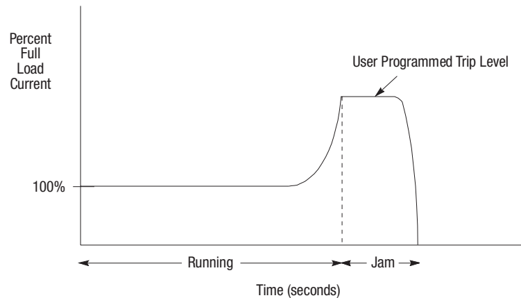
Figure 1.37: Jam Detection Sequence of Operation
