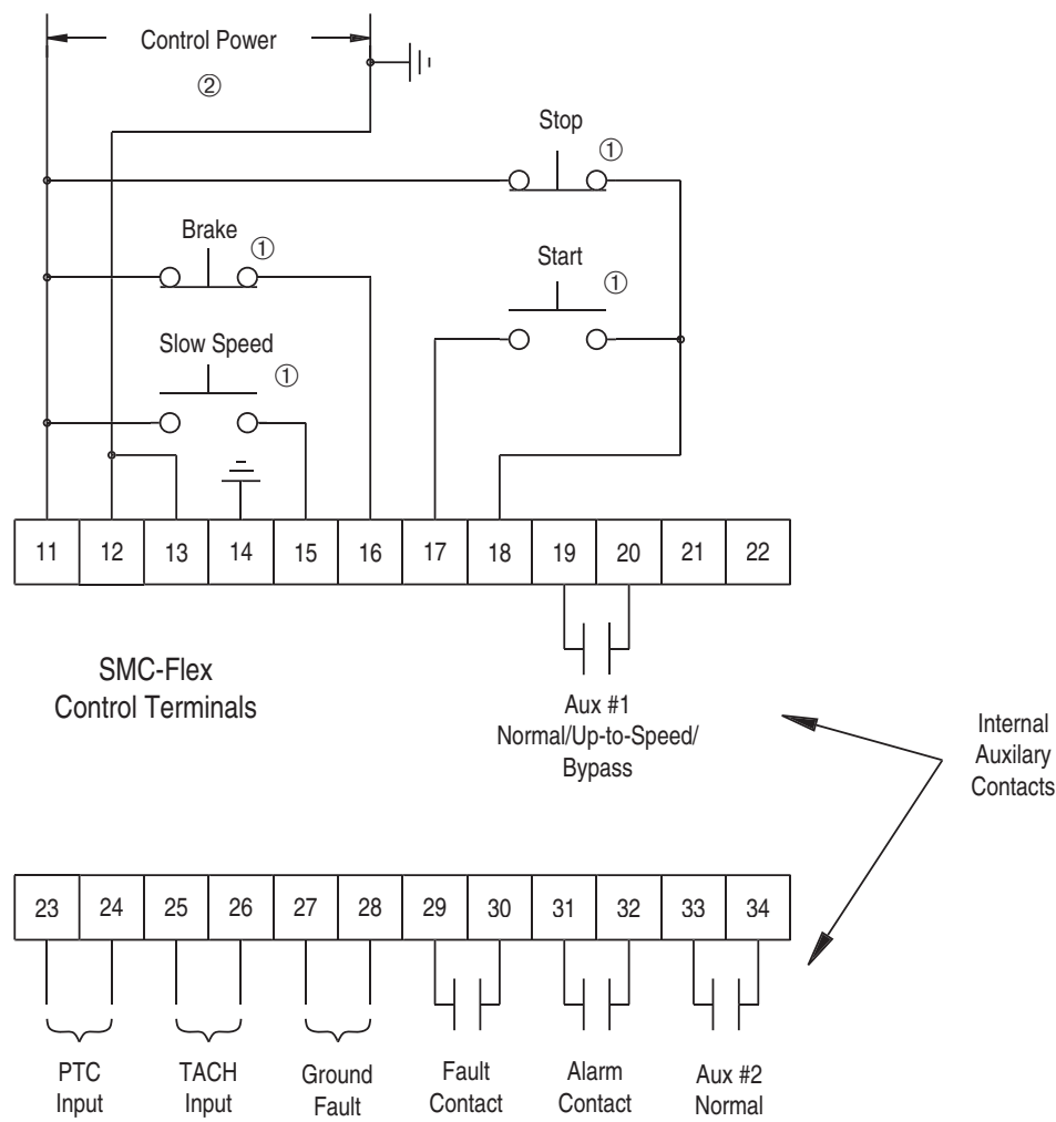
Figure 1.34: Slow Speed with Braking Wiring Diagram
