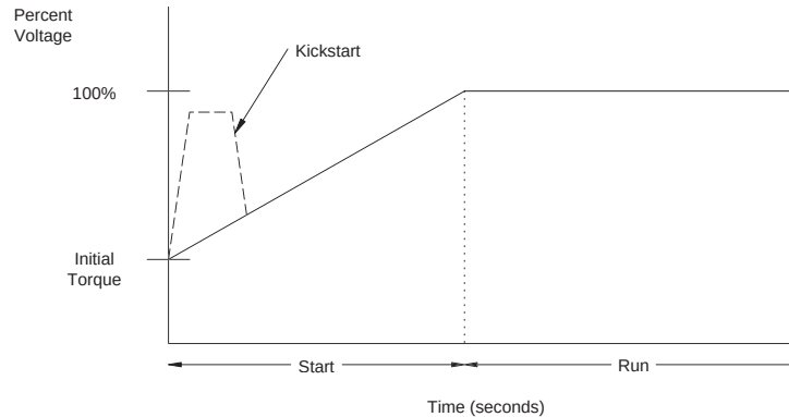
Figure 6.8: Soft Start
