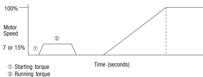
Figure 3.11: Starting and Running Torque
