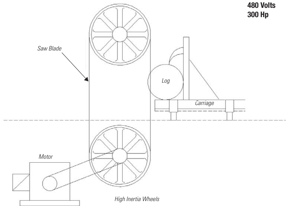
Figure 2.4: Bandsaw with Soft Start and Slow Speed with Braking
