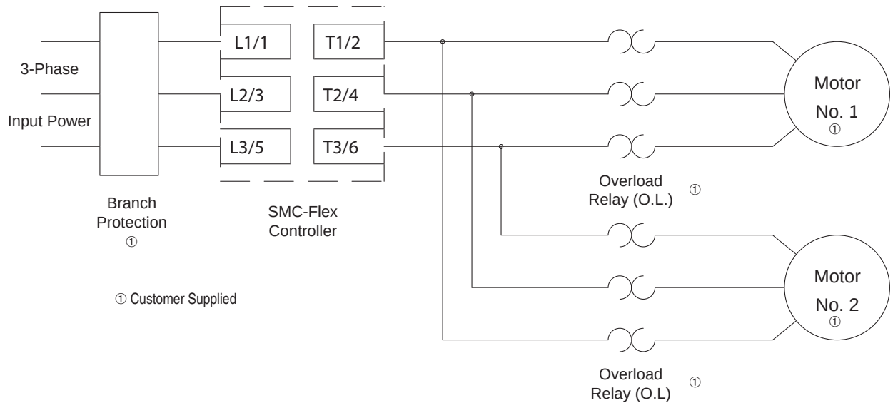
Figure 3.4: Multi-Motor Application
