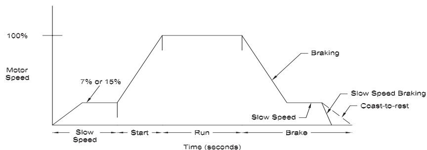
Figure 1.29: Accu-Stop
