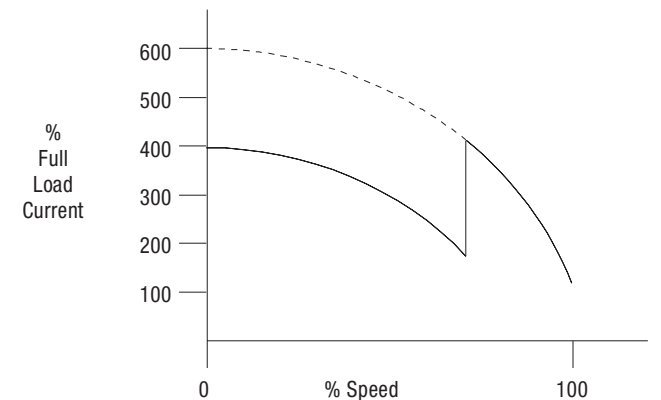
Figure 6.6: Transition near Full Speed
