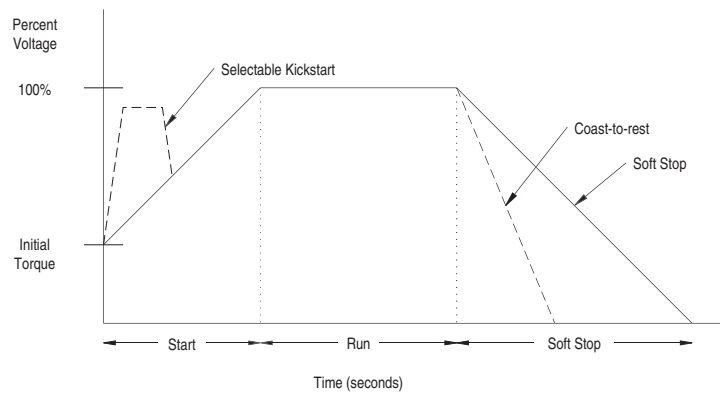
Figure 1.20: Soft Stop
