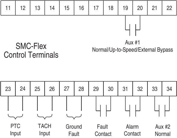
Figure 1.39: SMC-Flex Controller Control Terminals
